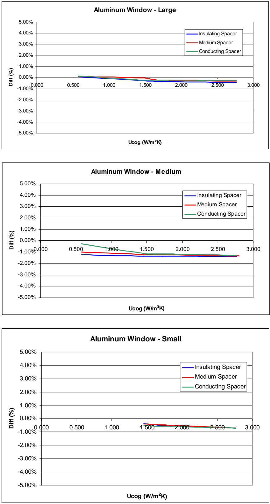
Figure 6.4-7: 3-D vs 2-D Differences for AL Window (Conduction models)
