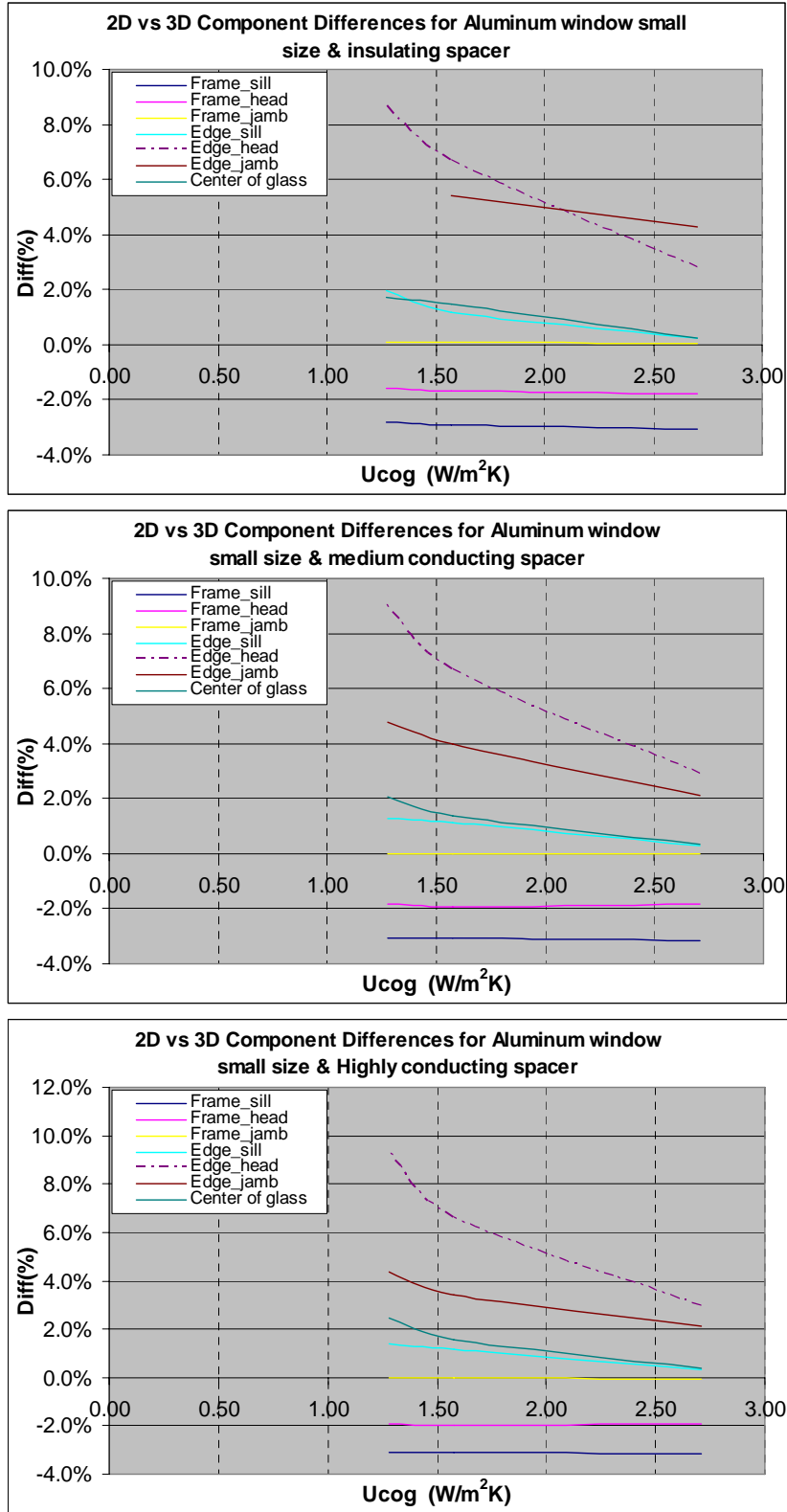
Figure 6.5-5: Component Level Difference Graphs for small Size Aluminum Window (convection models)
