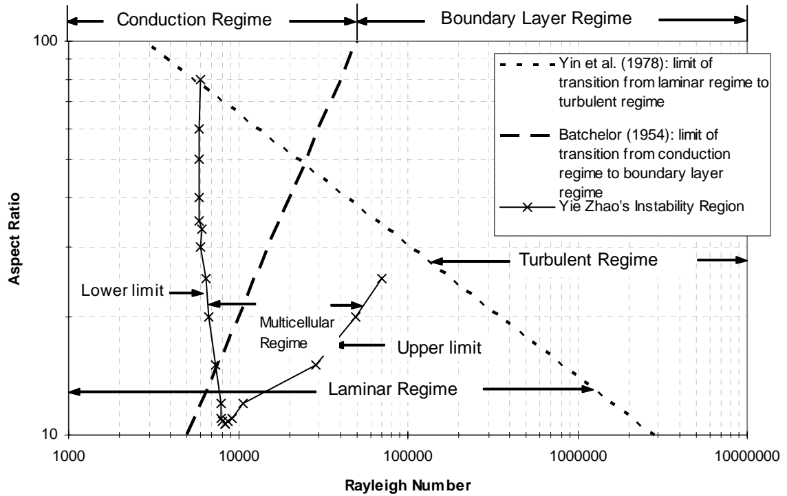
Figure 6.3-1: Definition of different flow regimes
