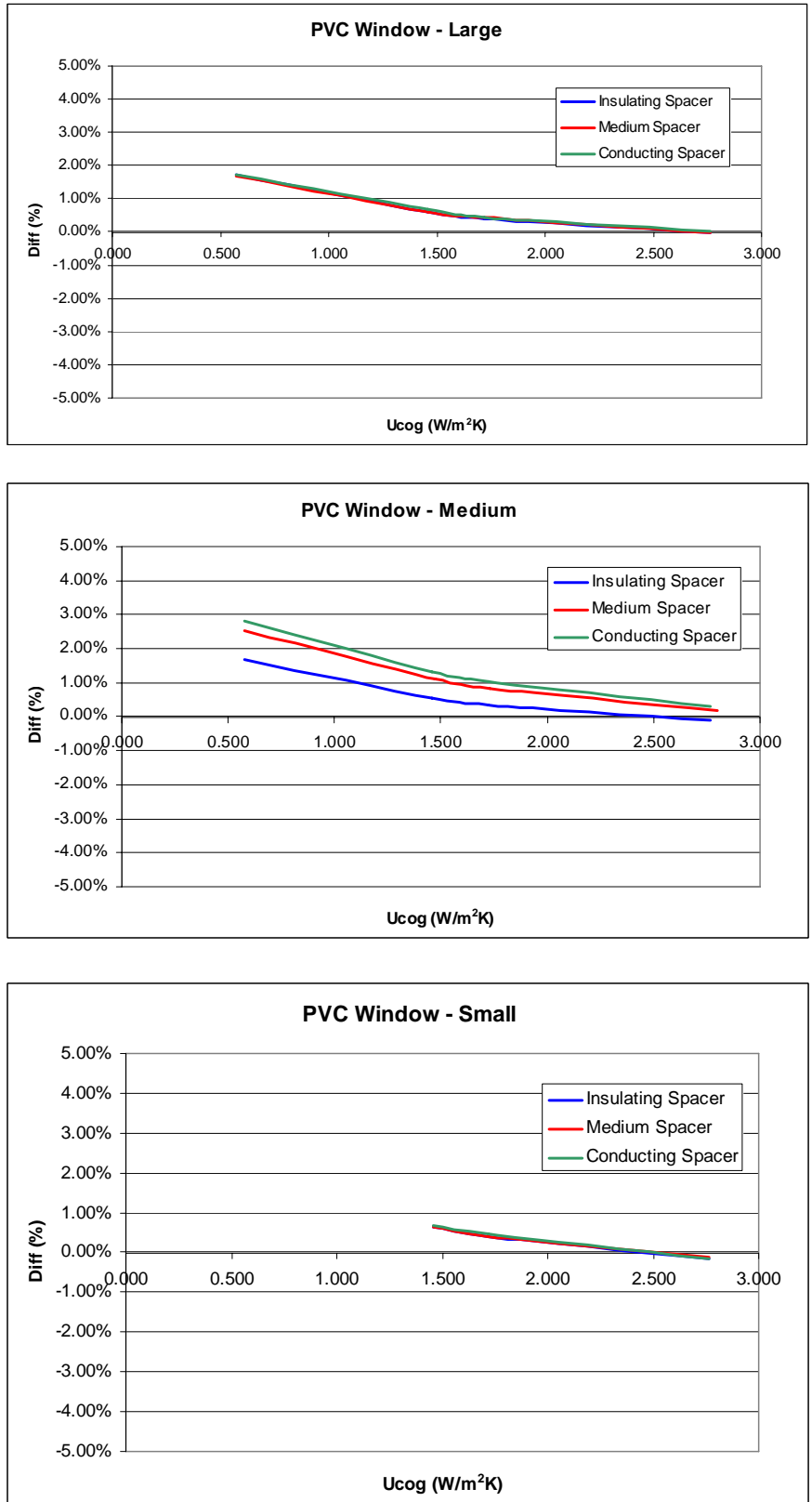
Figure 6.4-8: 3-D vs 2-D Differences for PVC Window (conduction Model)
