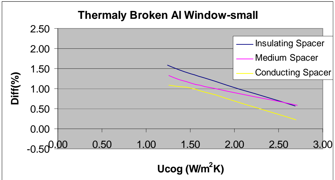
Figure 6.4-2: Overall 3-D vs 2-D Differences for T/B Al Window
