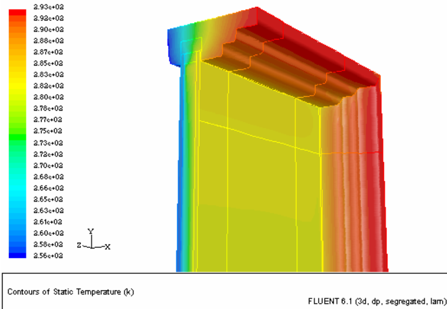
Figure B8: Temperature contour on the inside surface of Wood window - Convection model -3-d
