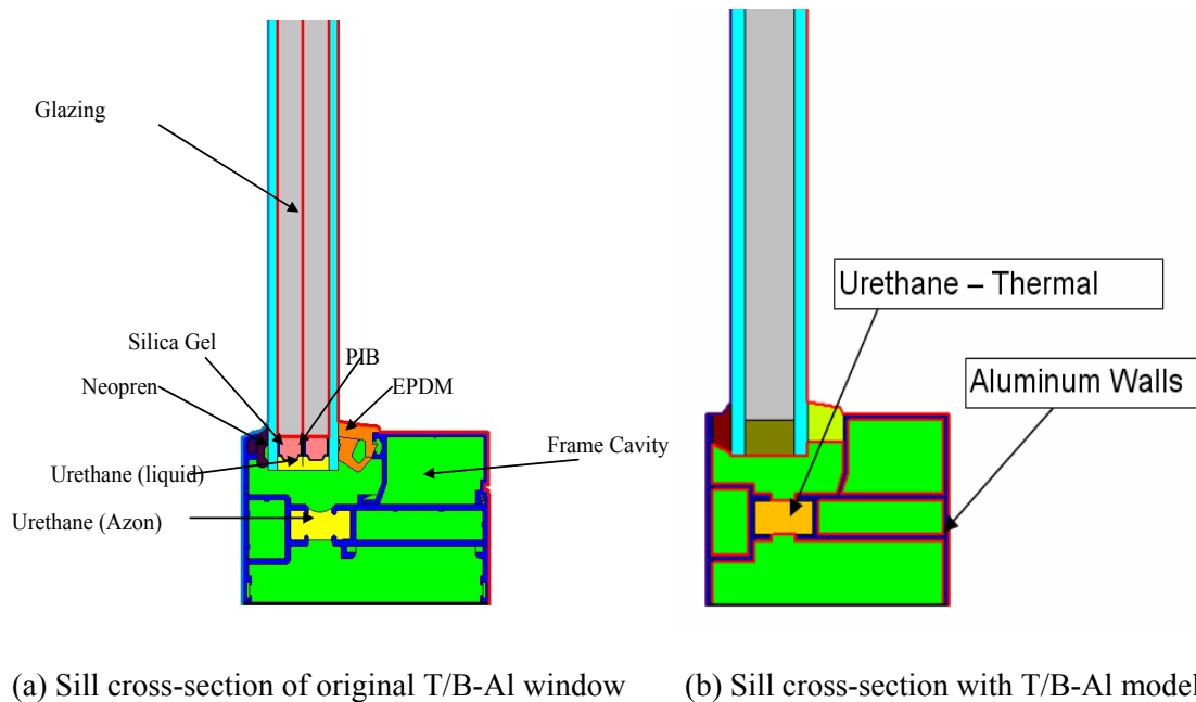
Figure 4.1-4: Sill cross-section view of TRR01 and T/B-Al windows
